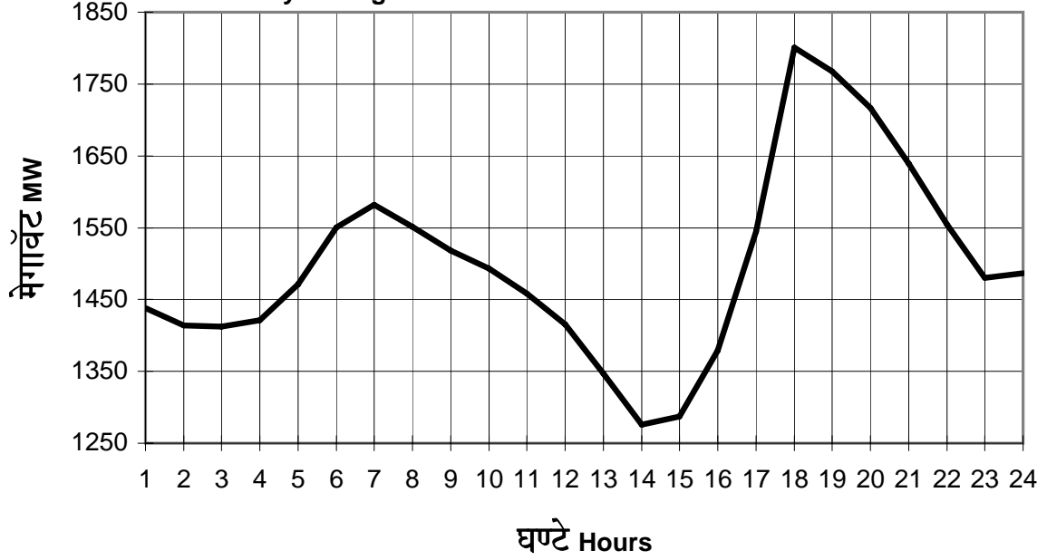
Hourly average CSEB Catered demand for Nov. 2007
