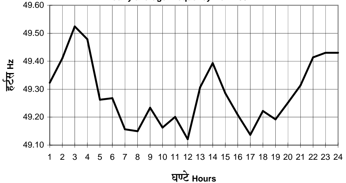
Hourly average Frequency Nov. 2007
