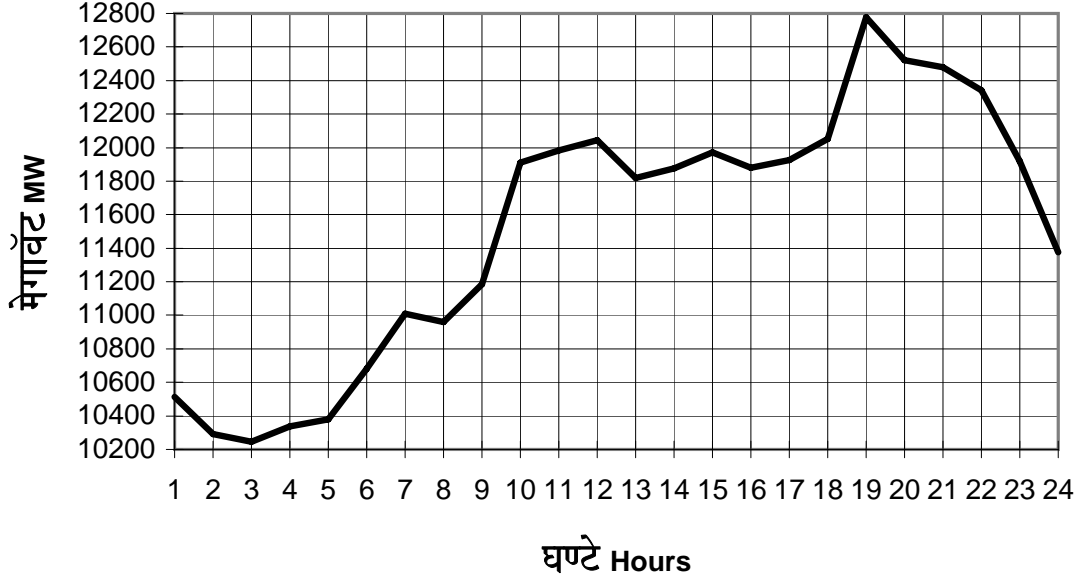
Hourly average Maharashtra Catered demand for Nov. 2007
