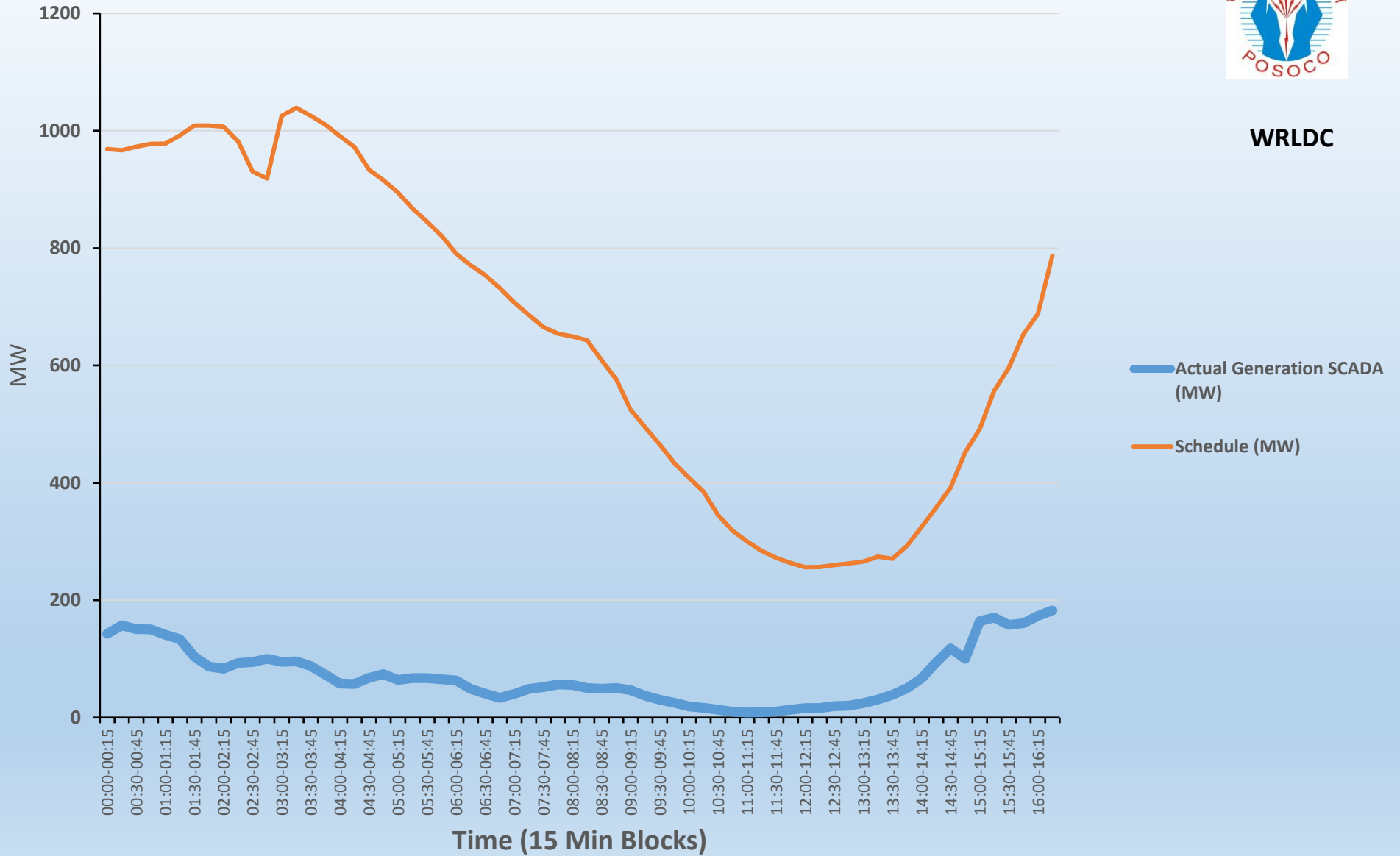
Schedule Vs Actual Wind Graph for 31-05-2017 Updated at 18:20
